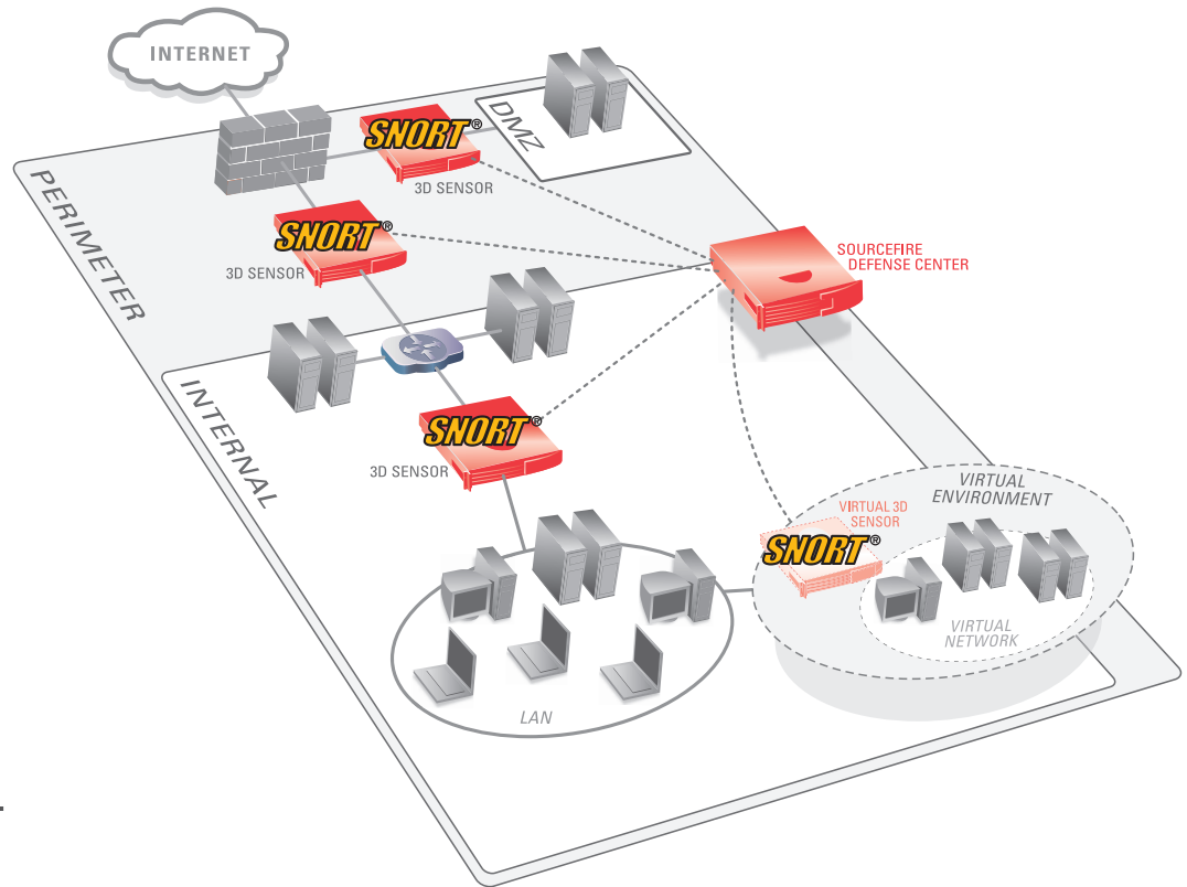
Figure 1. Sourcefire supports a Defense-in-Depth intrusion prevention strategy by allowing physical or virtual Sourcefire 3D Sensors to be positioned in all areas of the network. Sourcefire Defense Center orchestrates all event aggregation, analysis, and IPS policy management.
